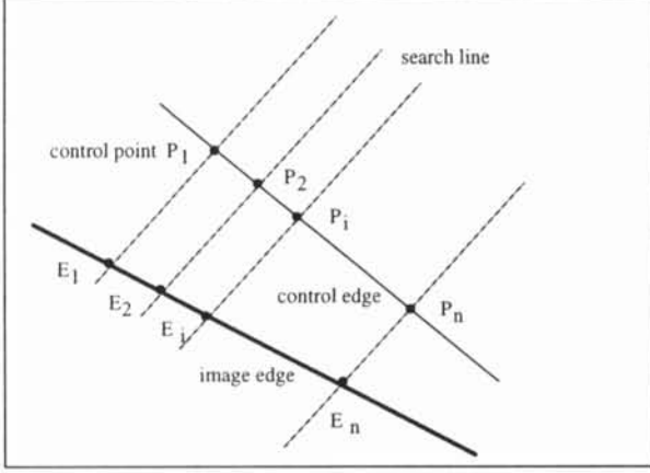
Figure 2: Detection of edge by minimizing image energy along search line.
