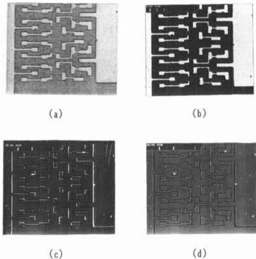
Fig.5 Example of inspection results for a mask sample pattern including random defects, erroneous pattern widths and some missing patterns
