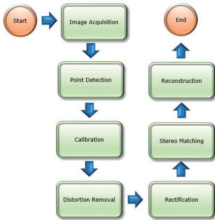
Figure 2. Calibrated Stereo Vision Pipeline
