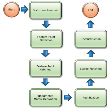
Figure 3. Uncalibrated Stereo Vision Pipeline
